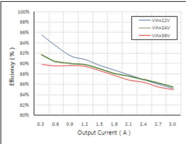
Figure 1, Efficiency
