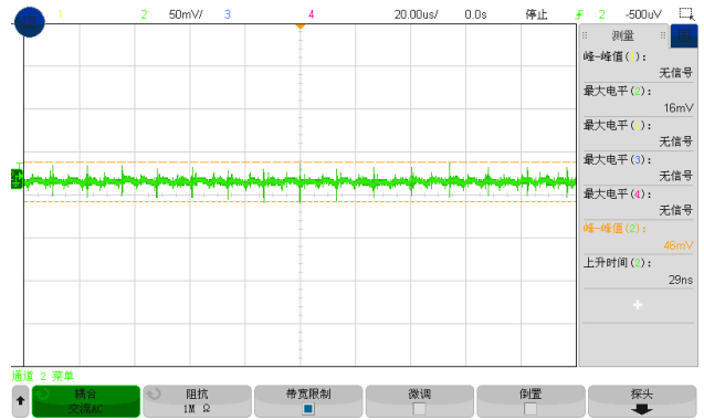
Figure 7, Output ripple & noise (Iout = 3A)
