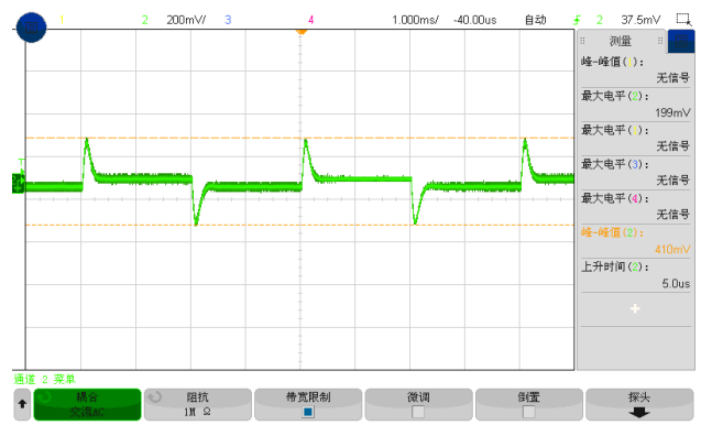
Figure 5, 50% - 75% load dynamic
