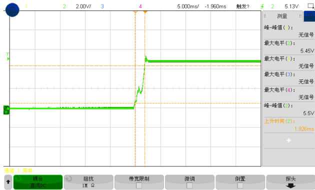
Figure 6, Output voltage established (Iout = 3A)
