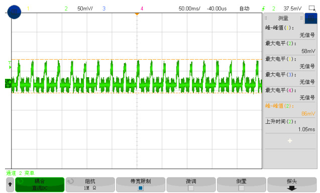
Figure 9, Short circuit & Out voltage (Iout = 3A)
