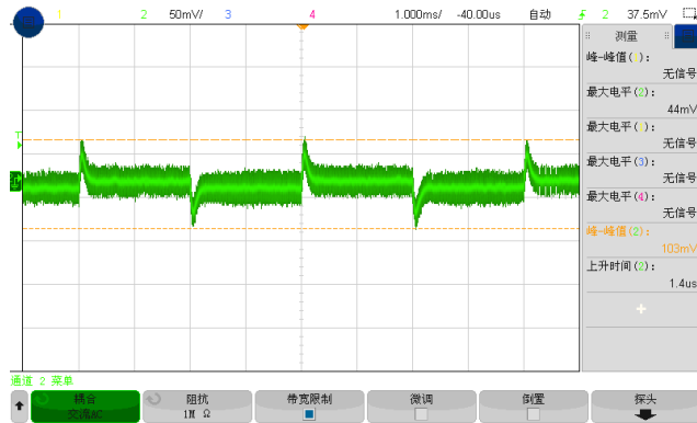
Figure 4, 25% - 50% load dynamic
