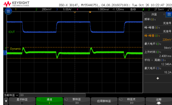
Figure 5, 50% - 75% load dynamic
