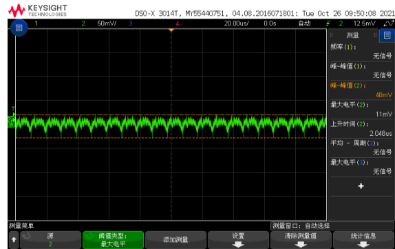
Figure 7, Output ripple & noise (Iout = 15A)
