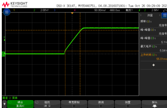
Figure 6, Output voltage established (Iout = 15A)
