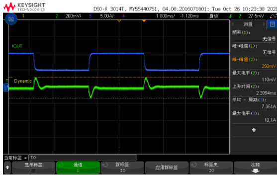
Figure 4, 25% - 50% load dynamic
